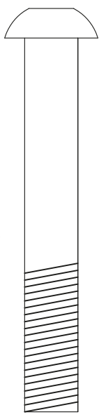
Inner hex bolt (M10*67) -4PCS
